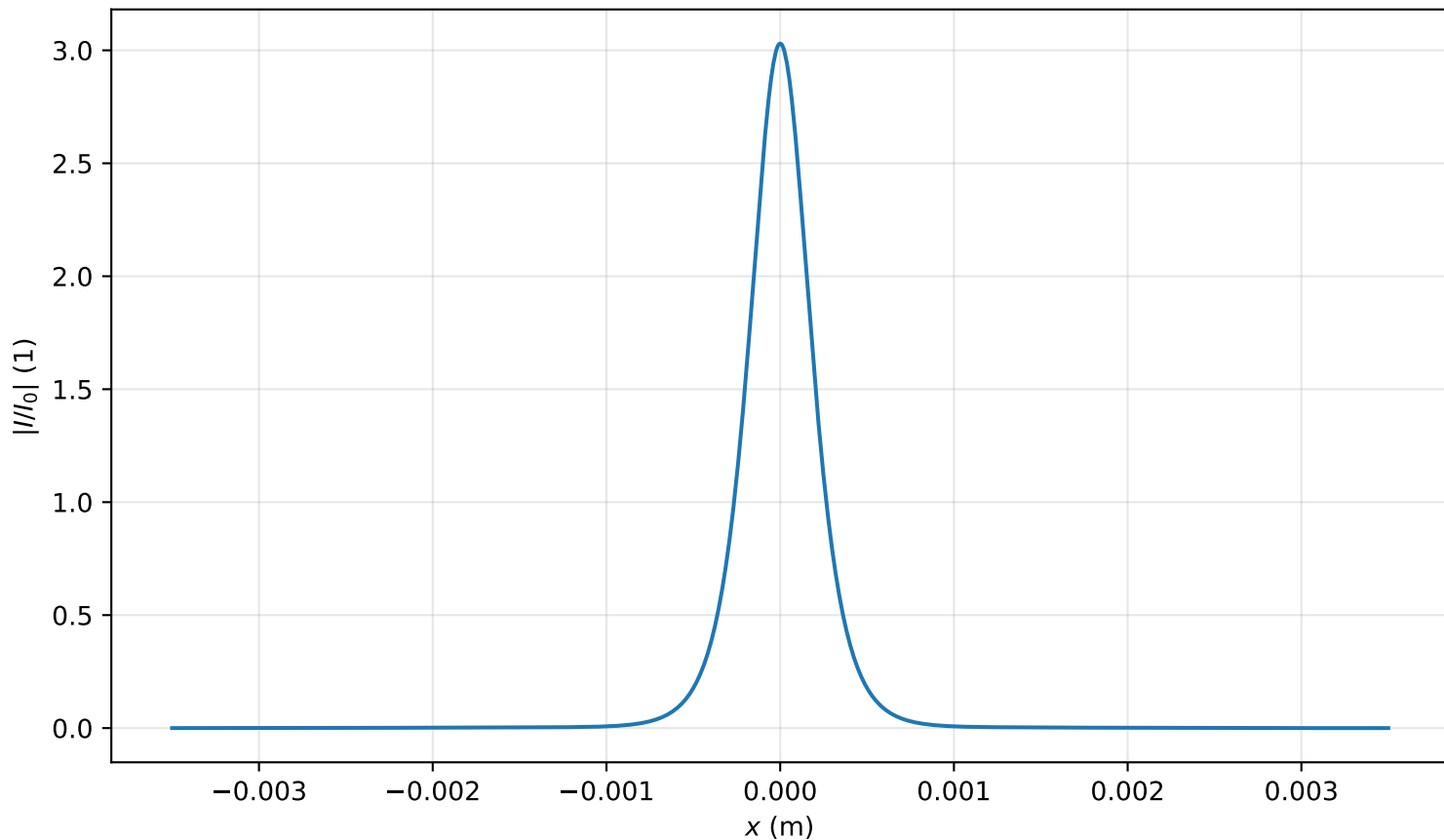
Intensity profile I(x, y = 0, z = 3.582m)/I_0 , P_{in}=1.0P_{cr} , artificial time
